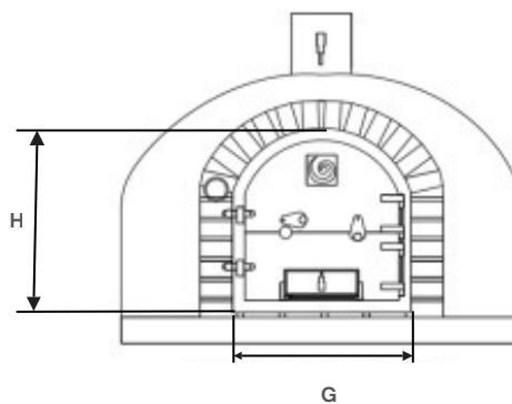
AOMR110 MISSION 44
